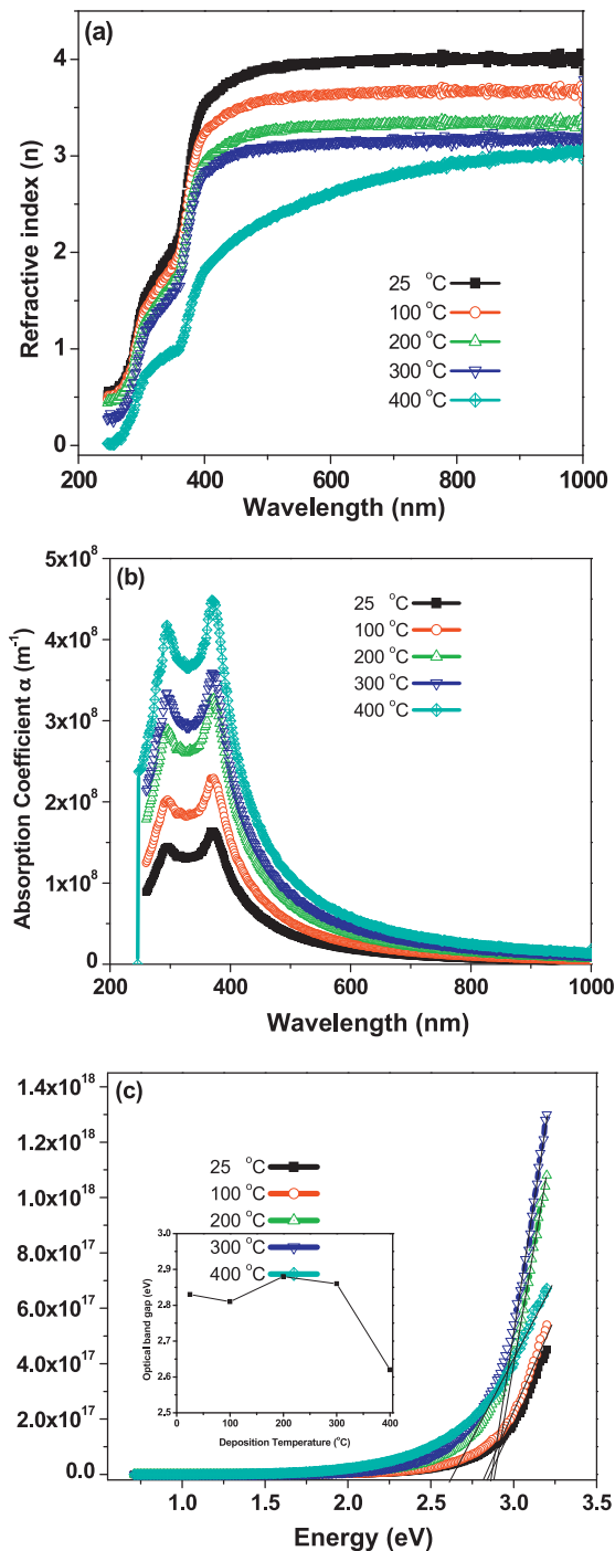
Fig. 3. Refractive index (a), absorption coefficient (b) as a function of wavelength, and plots of (ah\nu)^2 versus h\nu (c) of Al-doped CdO thin films deposited at different temperatures.
